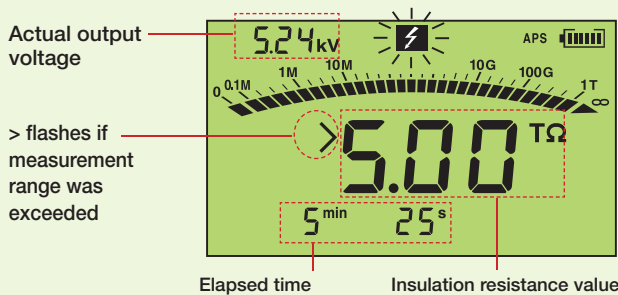
Insulation resistance measurement display
